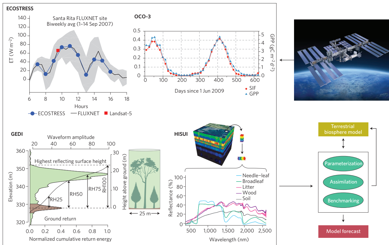
Figure 2 | A conceptual framework for how different data, observed from each ISS instrument, can be integrated into terrestrial biosphere models to improve their ability to represent and predict ecosystem processes. ECOSTRESS shows the 14-day average evapotranspiration (ET) from Santa Rita Fluxnet against the expected annual average value of ET from ECOSTRESS for each hour of the day. OCO-3 shows GOME solar-induced fluorescence data compared to the MPI-BGC gross primary productivity product. GEDI shows airborne LIDAR waveform from La Selva Biological Research Station, Costa Rica. HISUI shows an imaging spectroscopy/hyperspectral image cube and different spectra for different spectral classes. ISS image credit: Getty Images/sciabak.
