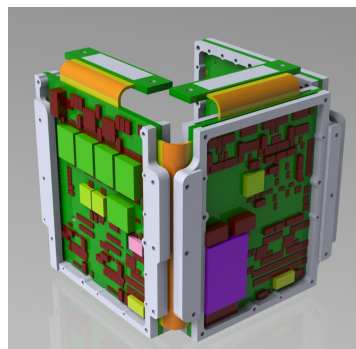
SpaceCube-Mini – IPEX
