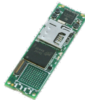
GumStix – IPEX
